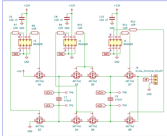
Main circuit
