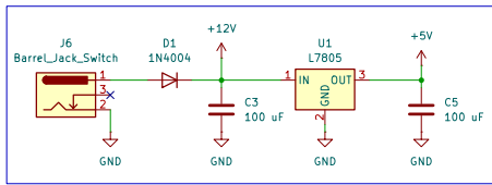
Power source
