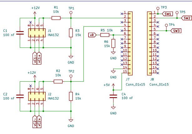
Instrumentation amplifiers and microcontroller
