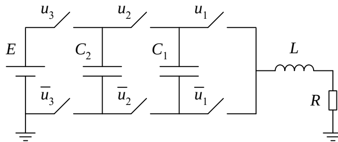
Figure 1: Circuit diagram.
