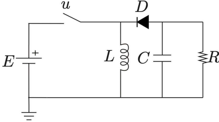
FIGURE 2.2 – Buck-Boos converter
