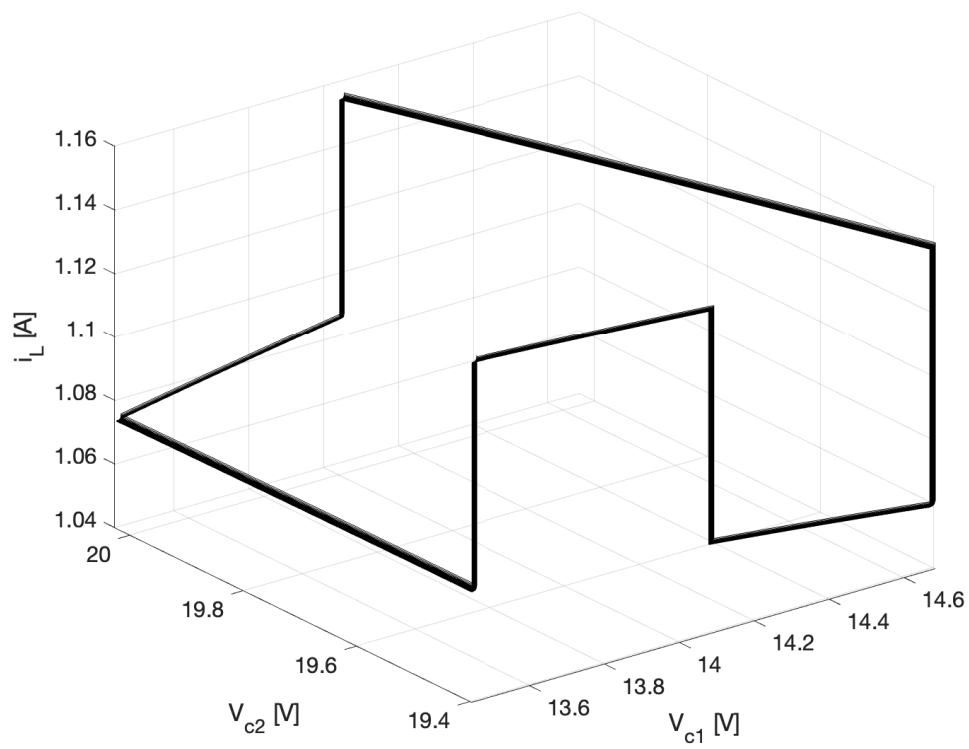
FIGURE 2.9 – Variant Dynamic Circuit 2: State Trajectory
