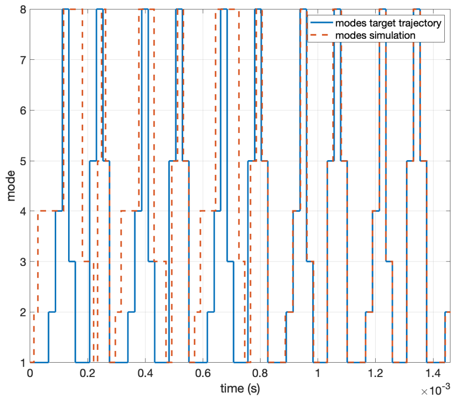
FIGURE 4.12 – Variant Dynamic Circuit 2: State Trajectory
