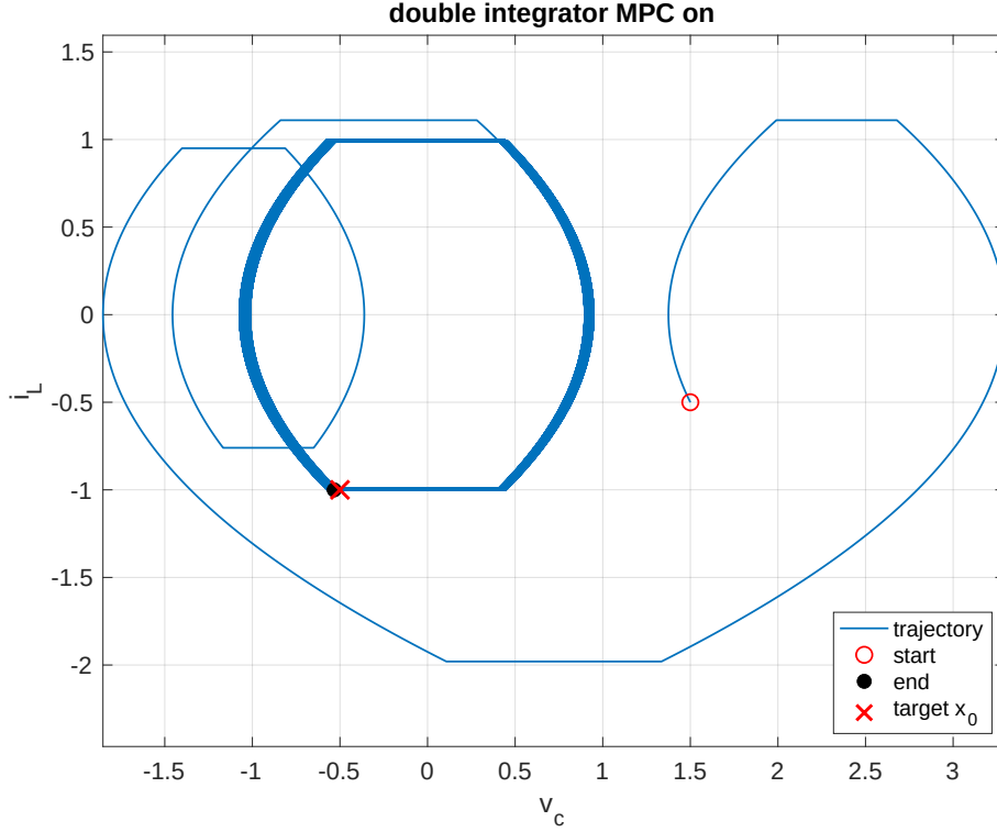
FIGURE 4.5 – State Trajectory MPC on, 50 cycles
