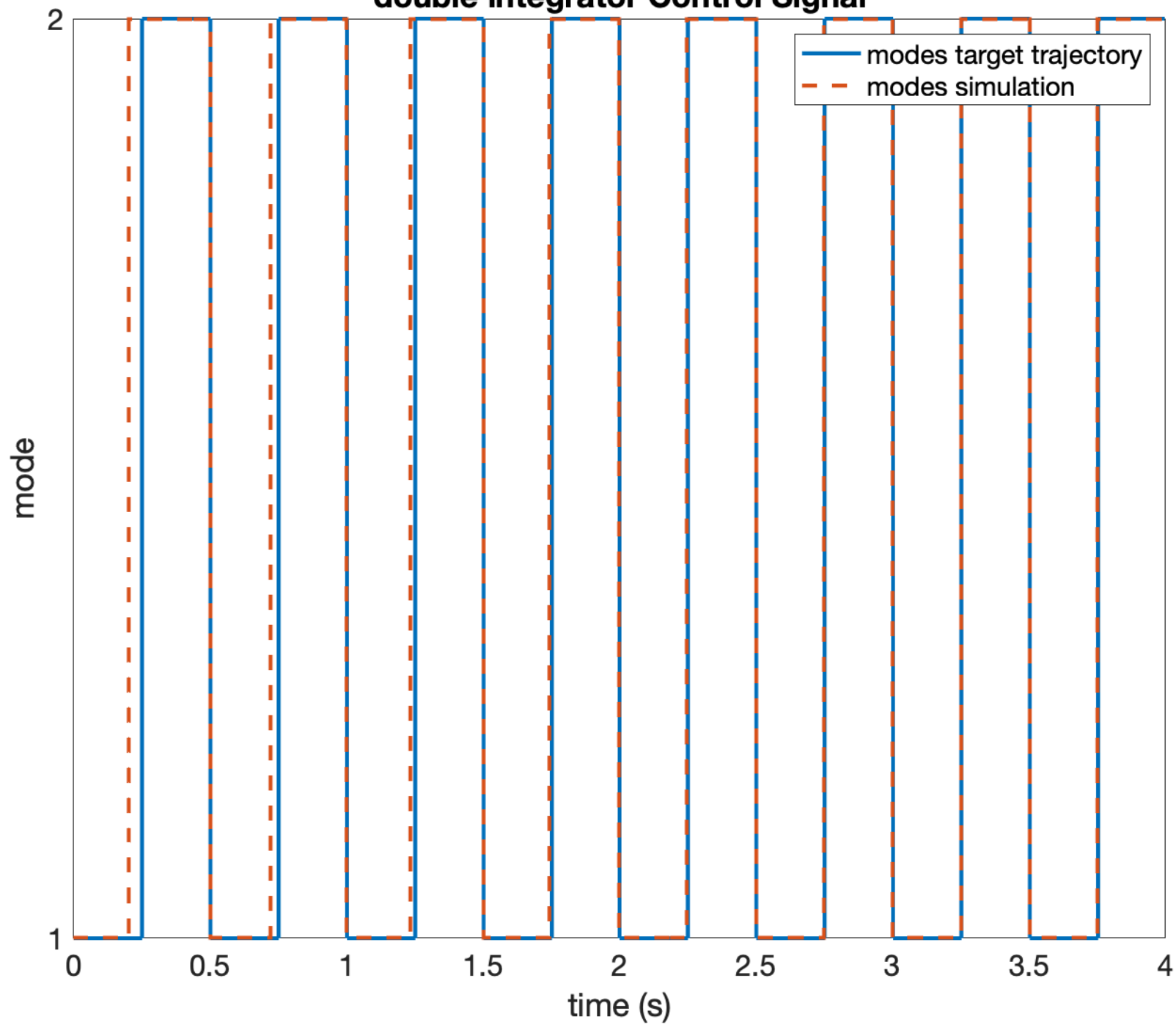
double integrator Control Signal
