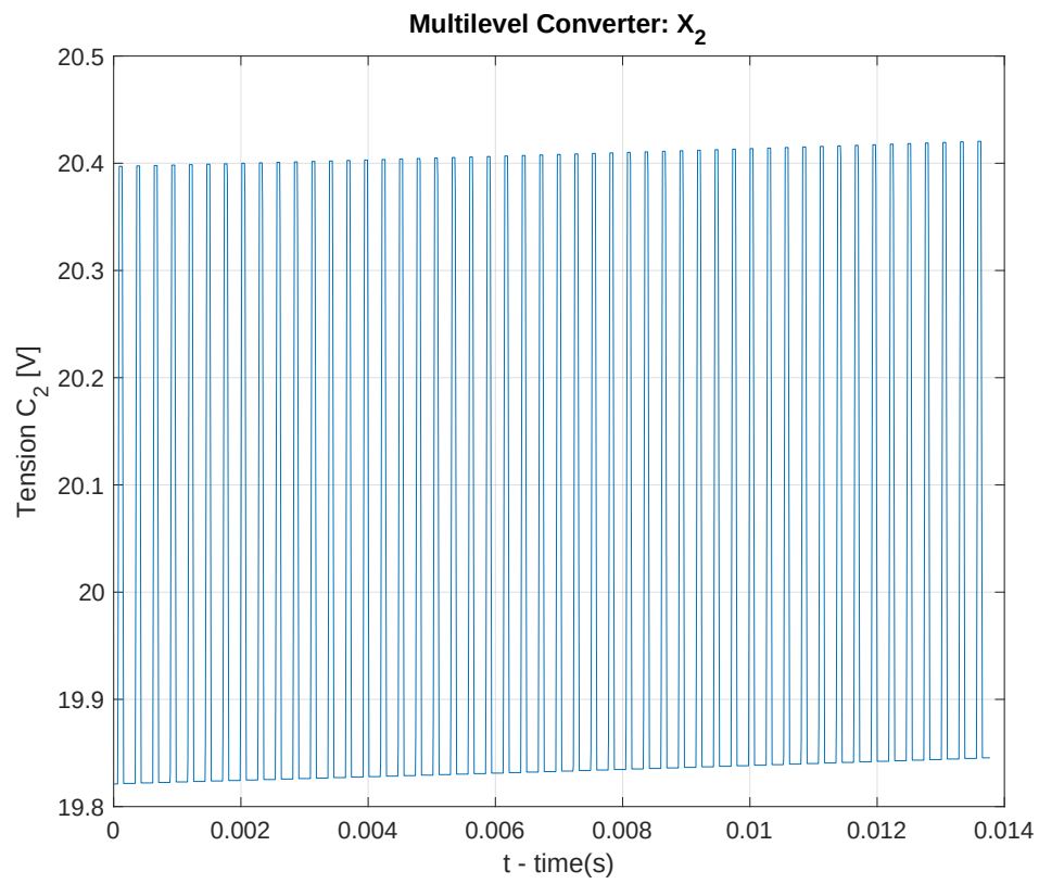
FIGURE 2.8 – Multilevel Converter: Voltage C_2
