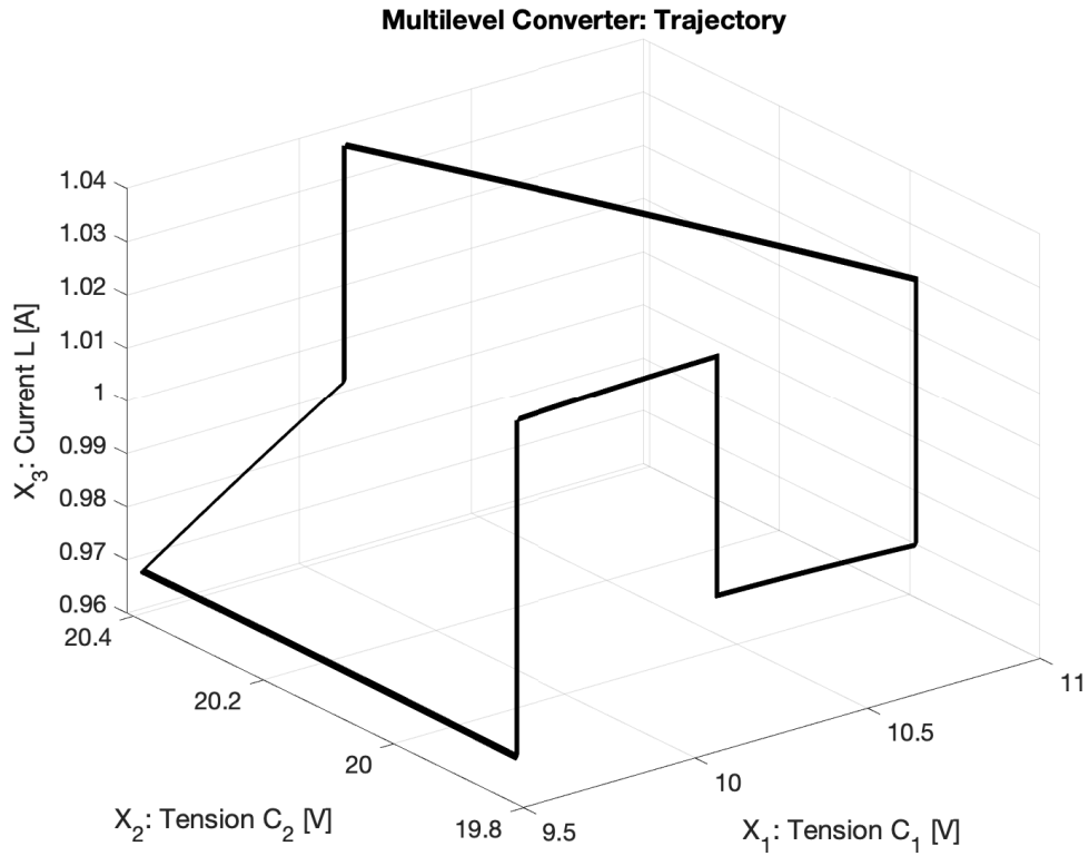
FIGURE 2.6 – Multilevel Converter: State Trajectory
