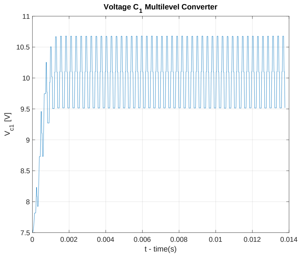
FIGURE 4.13 – Multilevel Converter: Voltage C_1
