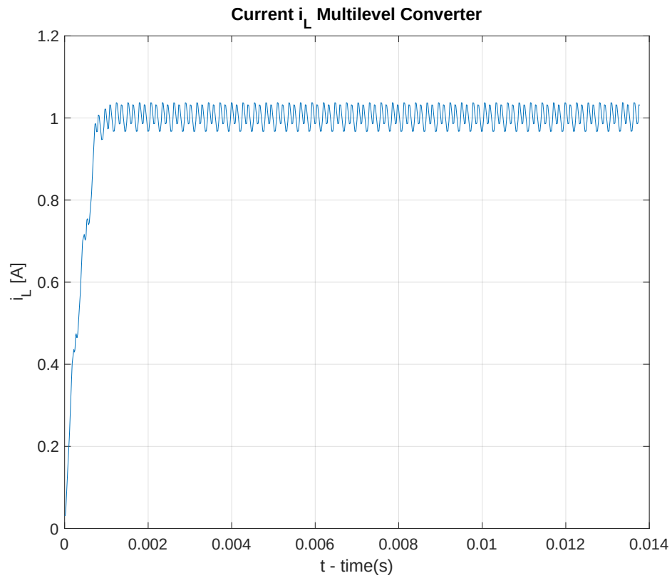
FIGURE 4.12 – Multilevel Converter: Current i_L
