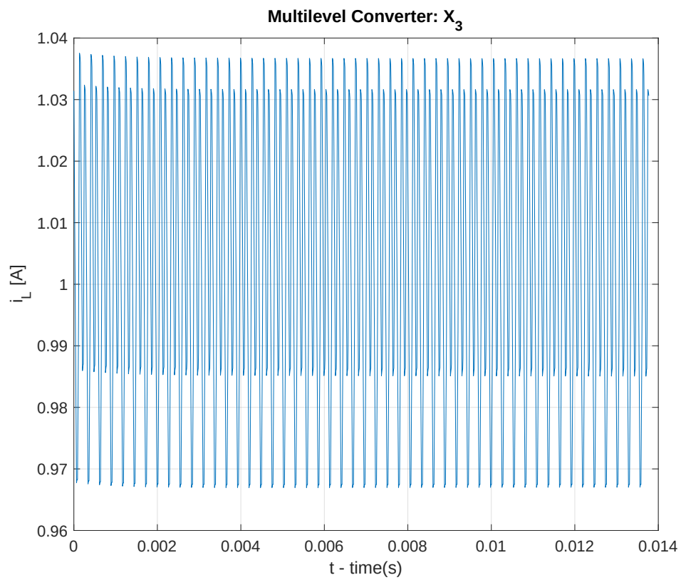
FIGURE 2.9 – Multilevel Converter: Current L
