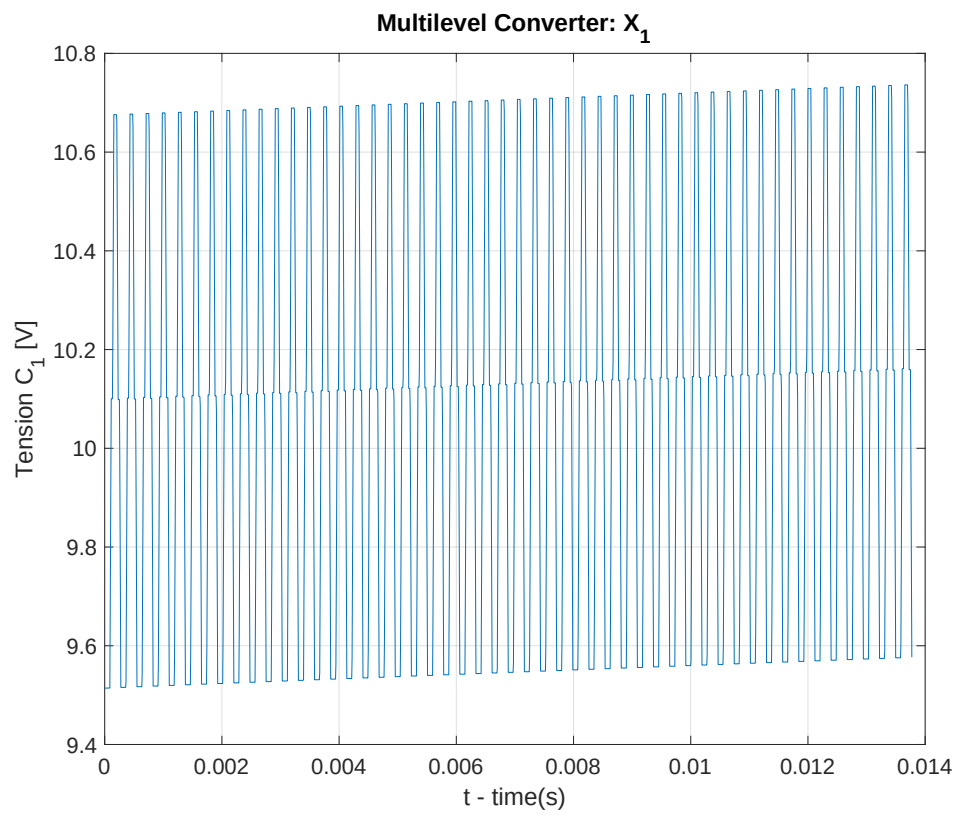
FIGURE 2.7 – Multilevel Converter: Voltage C_1
