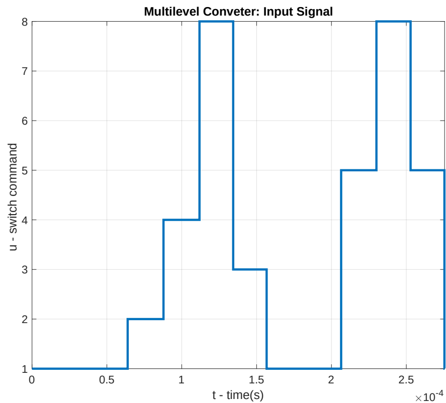
FIGURE 2.10 – Multilevel Converter: Input Signal
