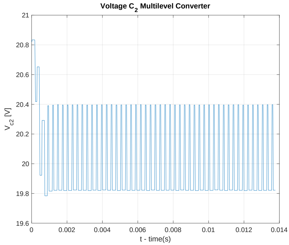
FIGURE 4.14 – Multilevel Converter: Voltage C_2
