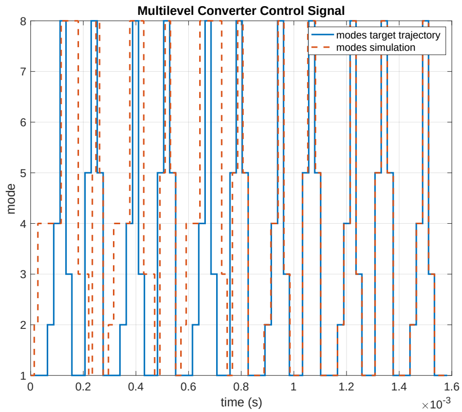
FIGURE 4.15 – Multilevel Converter: Control Signal
