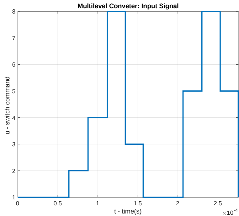
FIGURE 2.8 – Multilevel Converter: Input Signal
