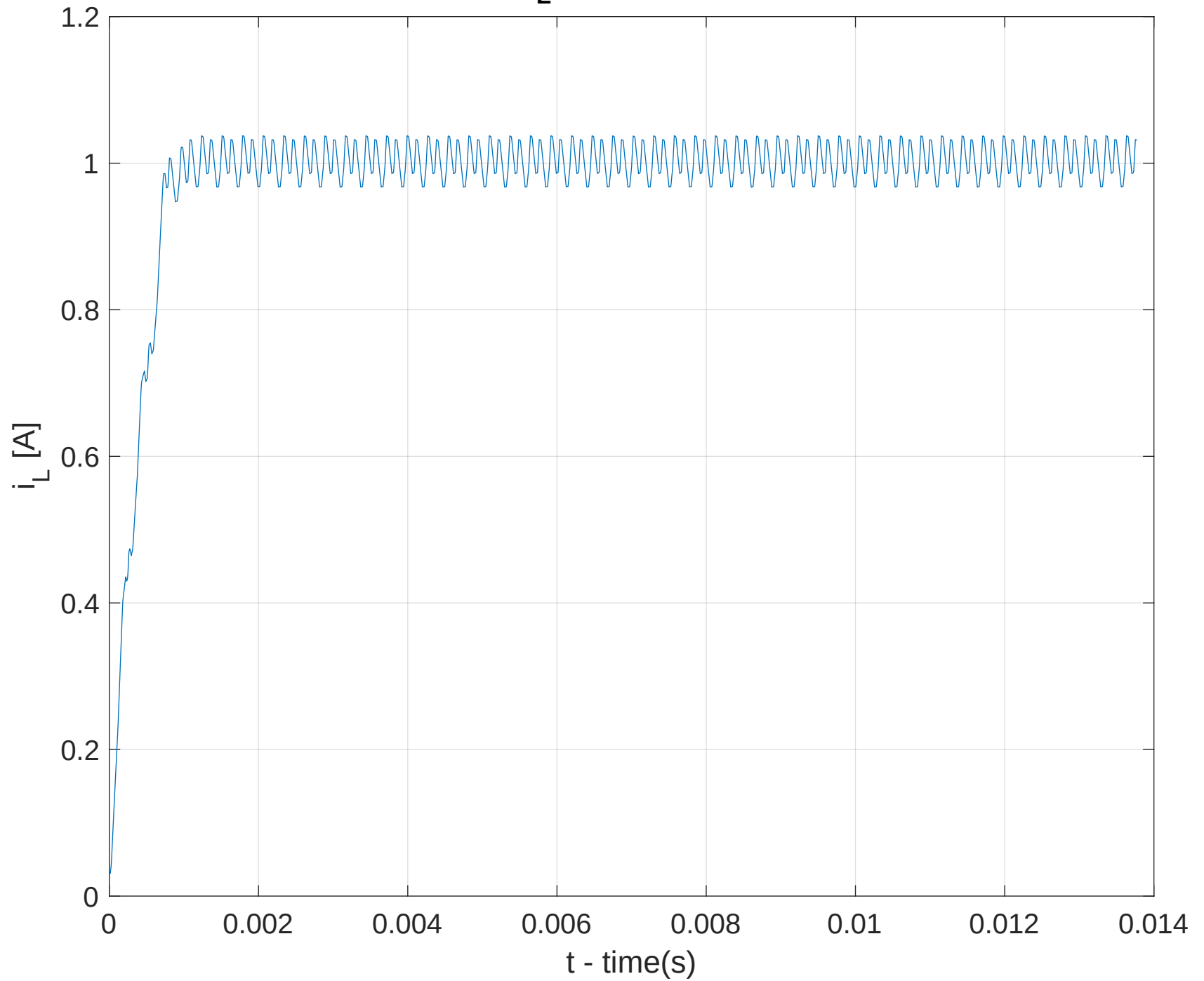
Current i_L Multilevel Converter
