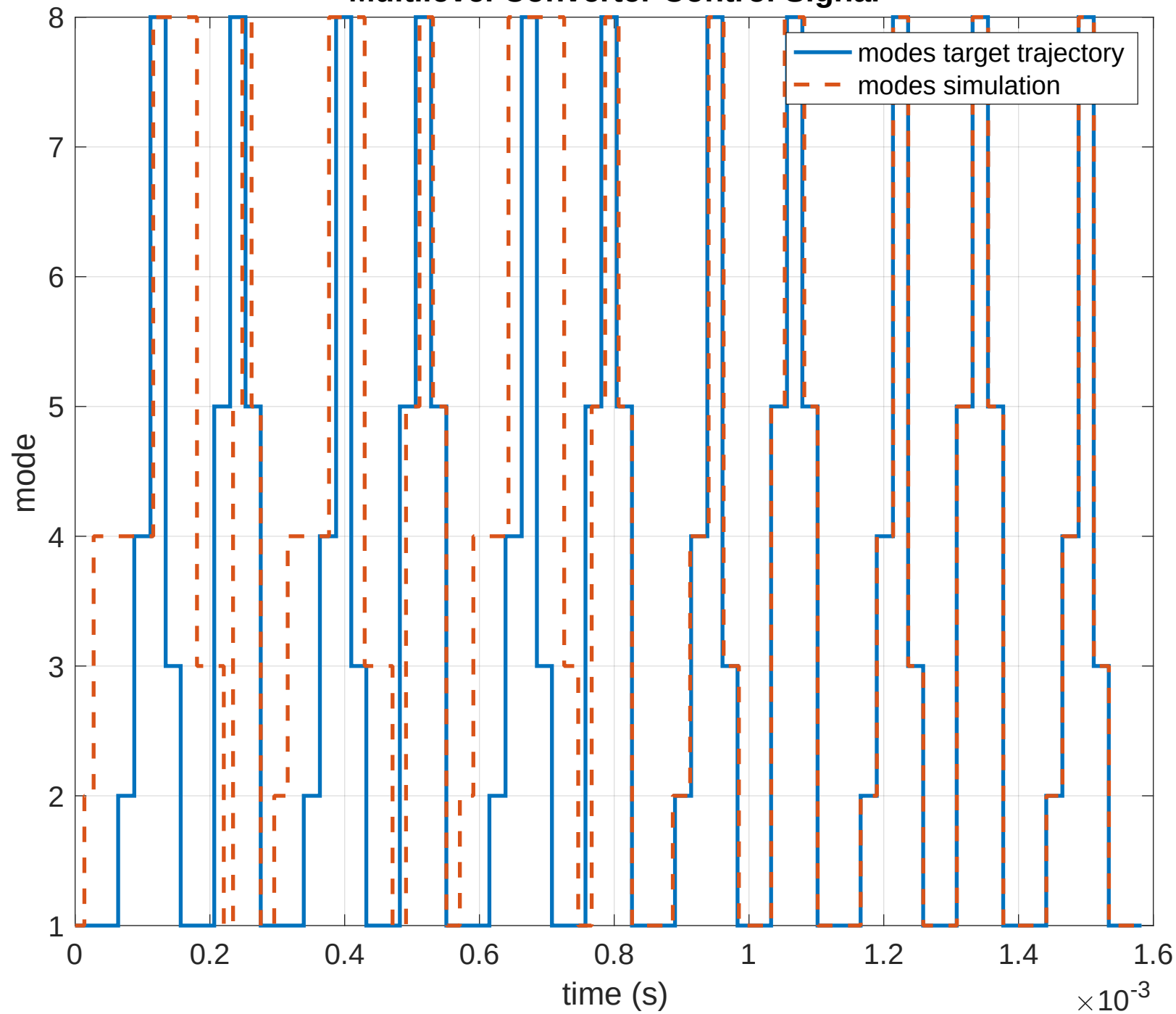
Multilevel Converter Control Signal
