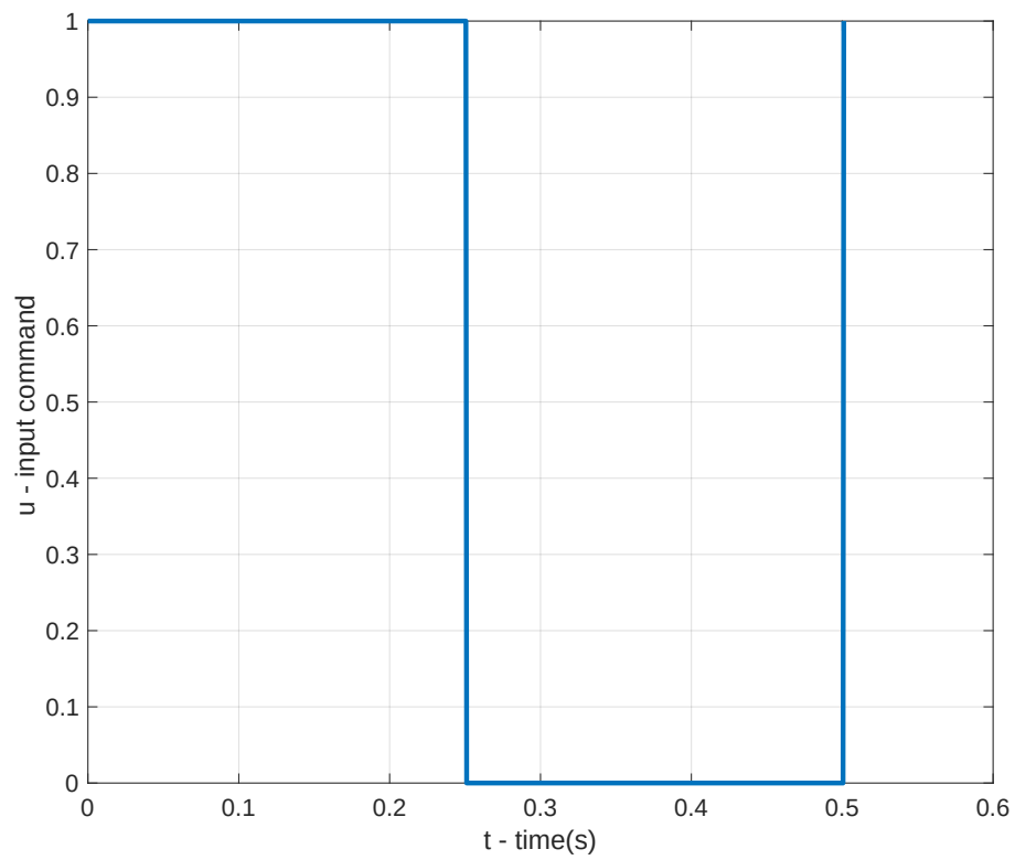
FIGURE 2.4 – Buck-Boost converter: Switch command
