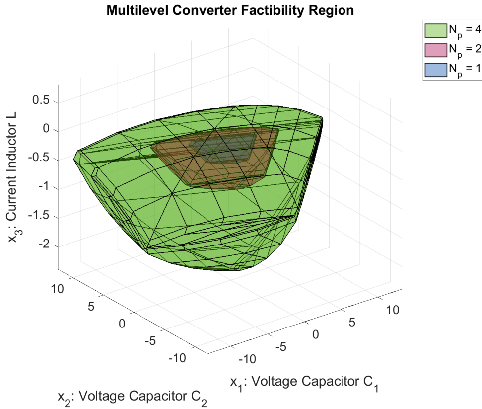
FIGURE 4.13 – Multilevel Converter: Feasibility Region
