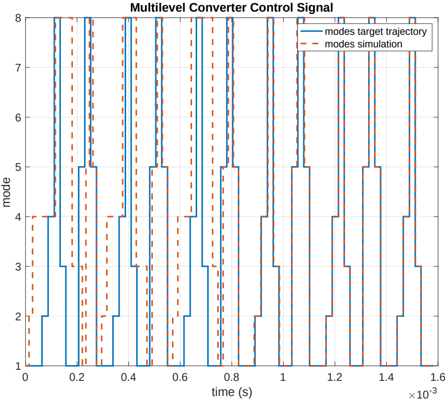
FIGURE 4.17 – Multilevel Converter: Control Signal
