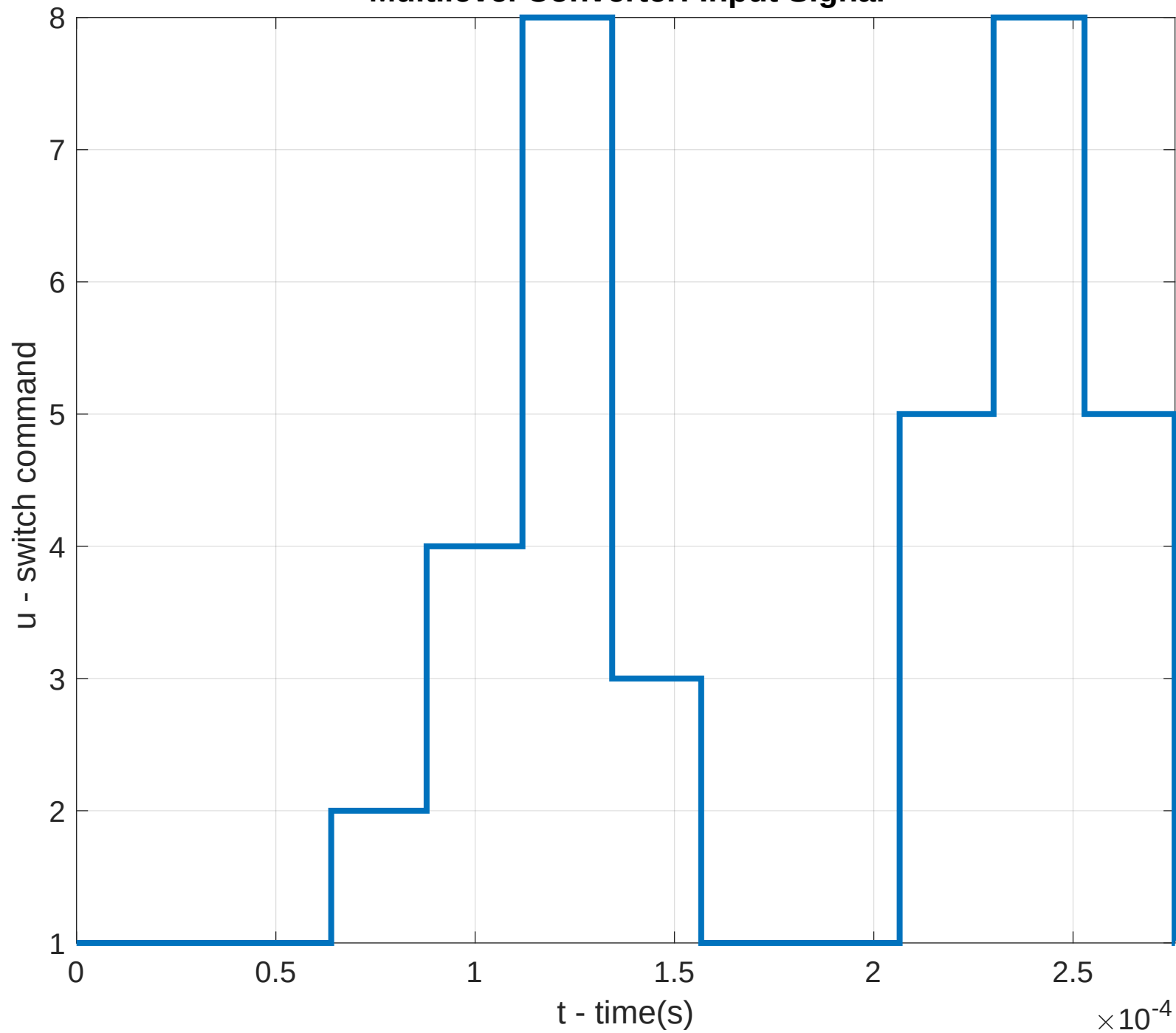
Multilevel Converter: Input Signal
