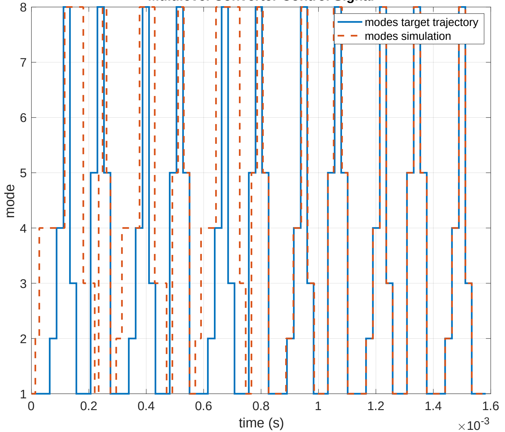
Multilevel Converter Control Signal
