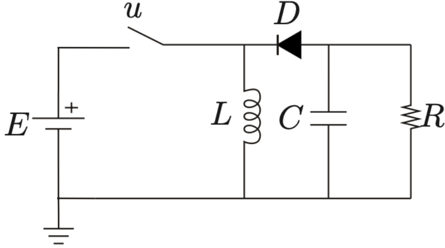
FIGURE 2.2 – Buck-Boos converter
