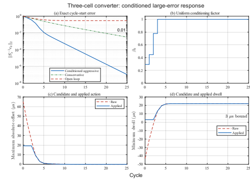
Figure 3 Exact nonlinear response from the large-error initial state, showing the first 25 of the 100 simulated cycles. (a) Normalized cycle-start errors with conditioned aggressive feedback, unconditioned conservative feedback, and open loop. (b) Conditioning factor. (c) Maximum absolute raw and applied switching-instant offsets. (d) Minimum raw and applied dwell durations. The raw duration becomes negative, while the applied schedule satisfies the assumed 3 \mu\text{s} bound.
