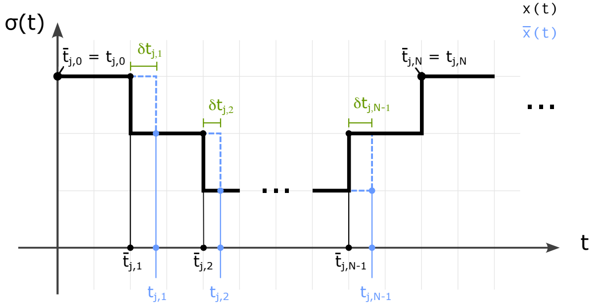
FIGURE 4.1 – Input signals
