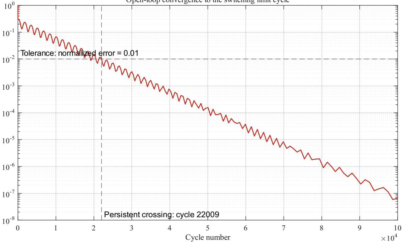
Open-loop convergence to the switching limit cycle
