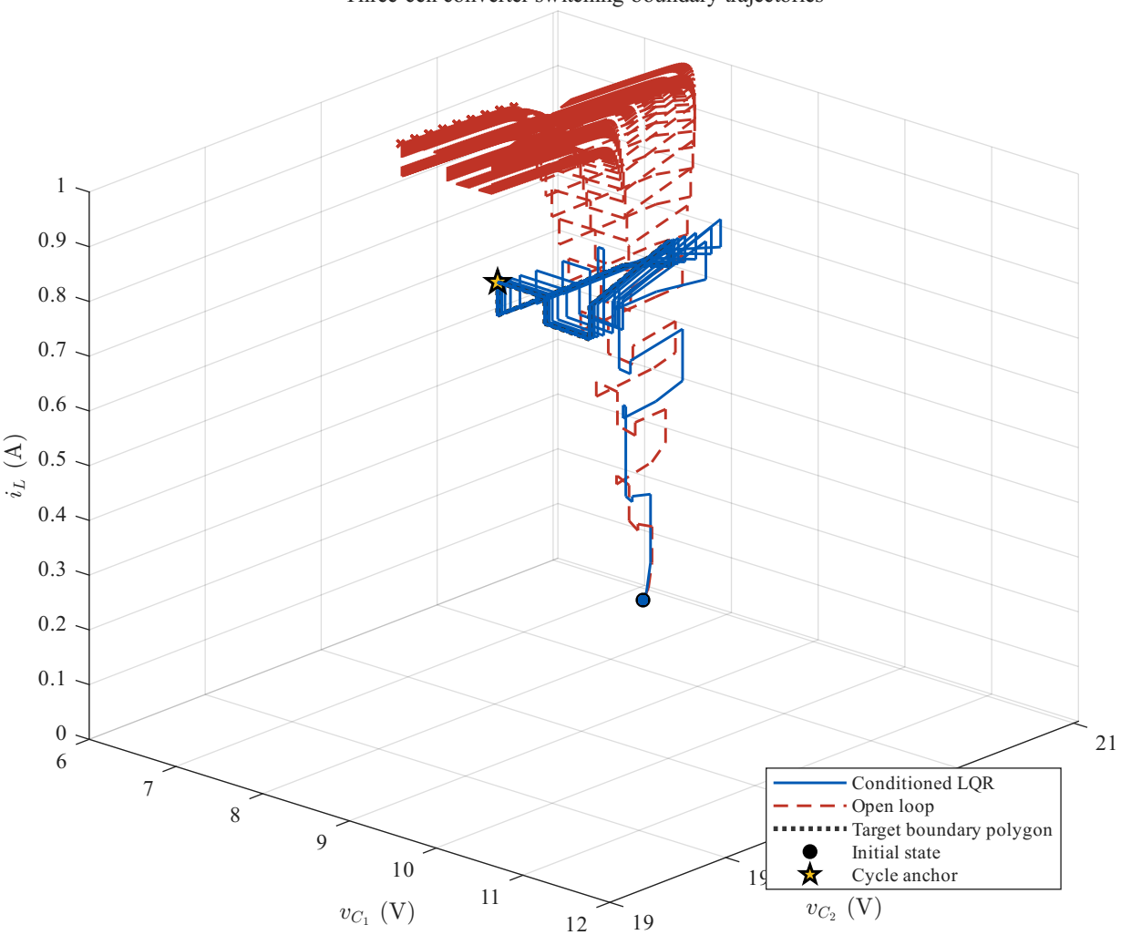
Three-cell converter switching-boundary trajectories
