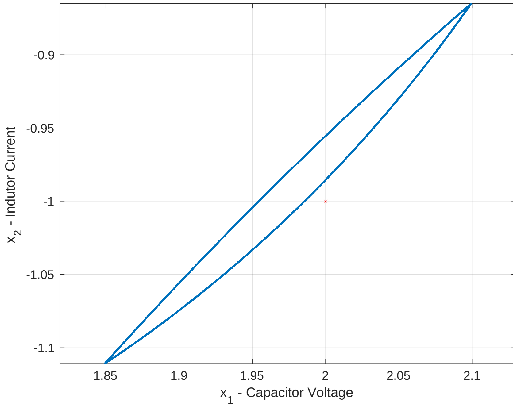
Buck-Boost Converter: Cyclic Trajectory
