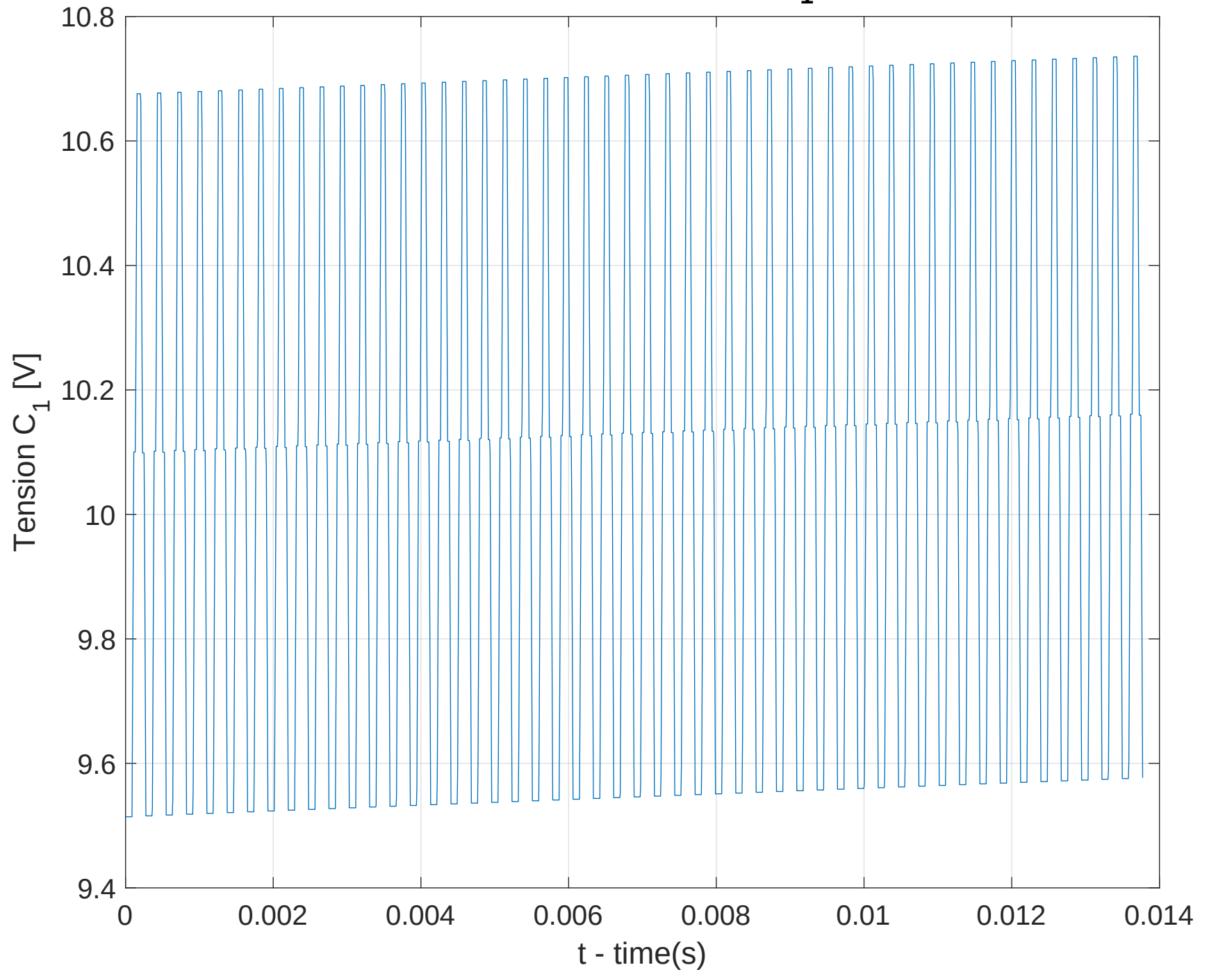
Multilevel Converter: X_1
