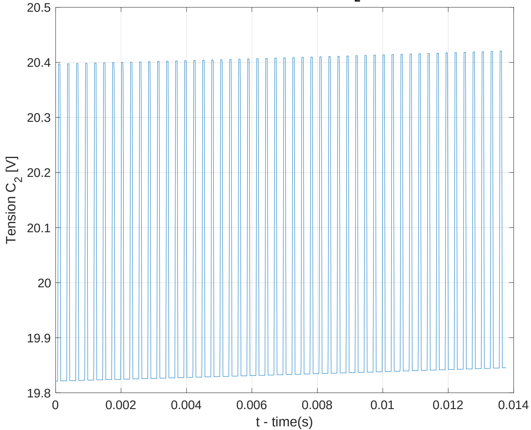
Multilevel Converter: X_2
