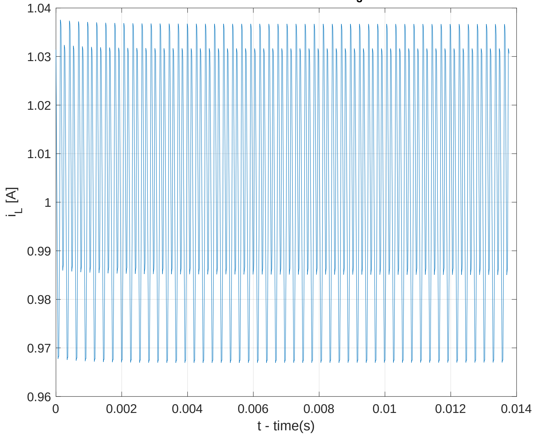
Multilevel Converter: X_3
