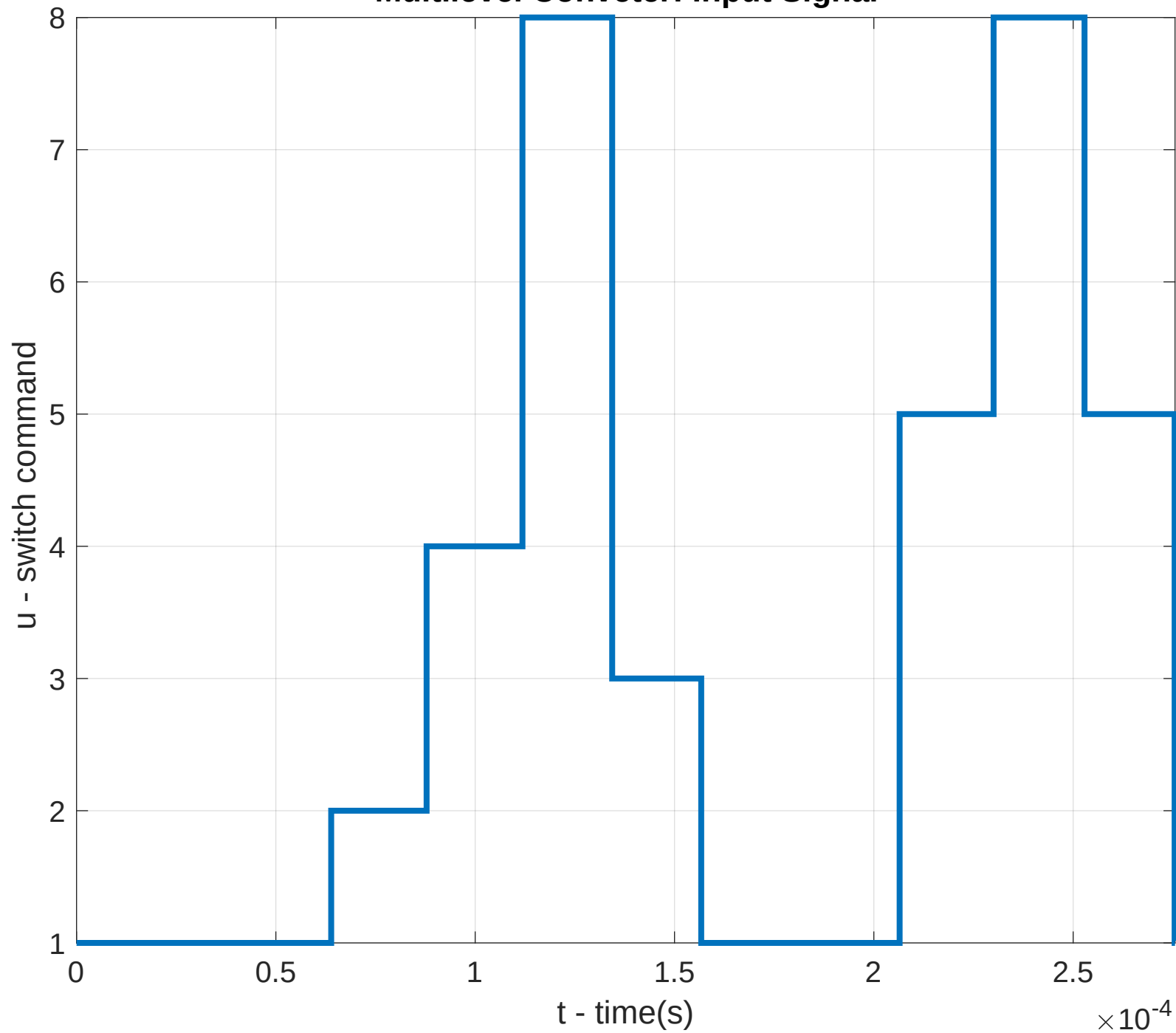
Multilevel Conveter: Input Signal
