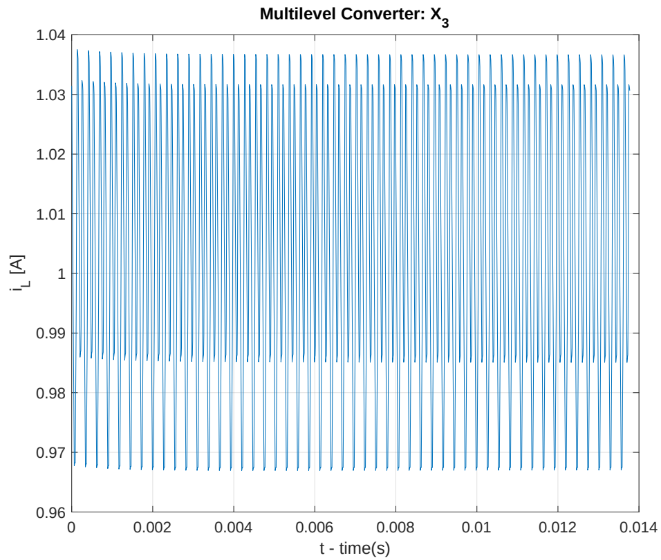
FIGURE 2.8 – Variant Dynamic Circuit 2: Current L
