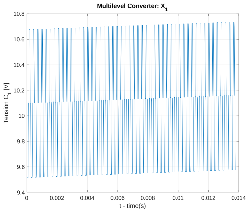
FIGURE 2.6 – Variant Dynamic Circuit 2: Voltage C_1
