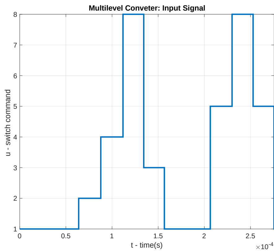
FIGURE 2.10 – Variant Dynamic Circuit 2: Input Signal
