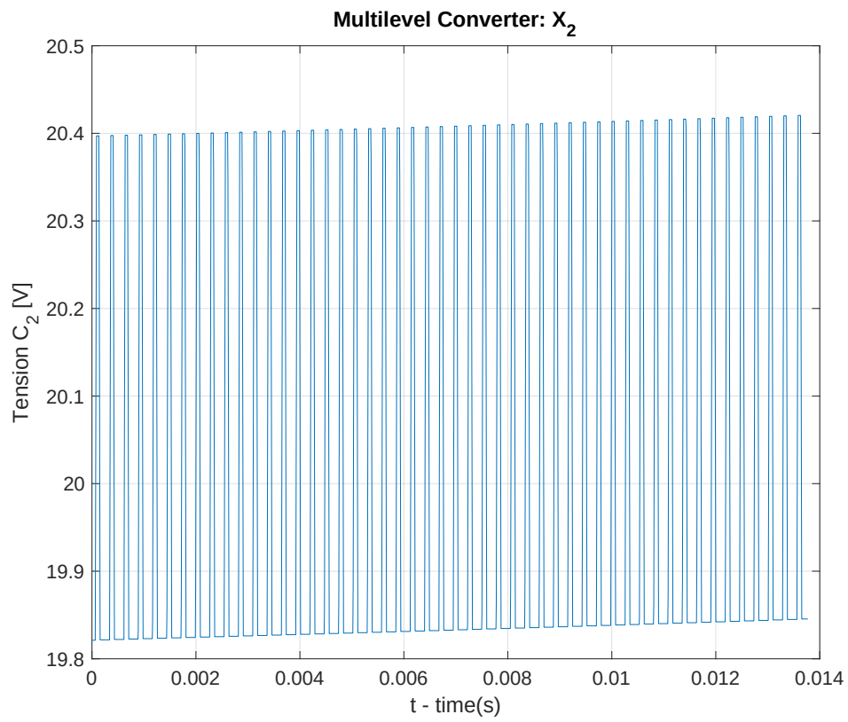
FIGURE 2.7 – Variant Dynamic Circuit 2: Voltage C_2
