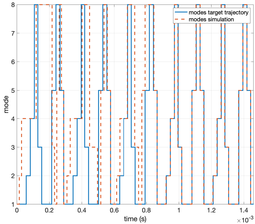
FIGURE 4.8 – Variant Dynamic Circuit 2: State Trajectory
