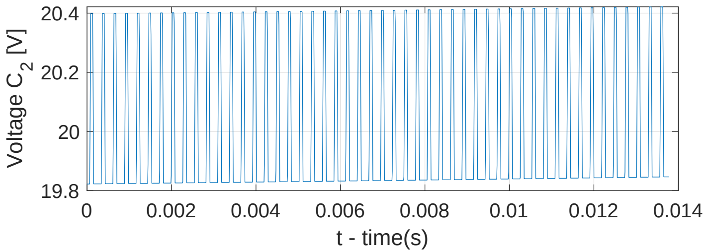
Multilevel Converter: X_3
