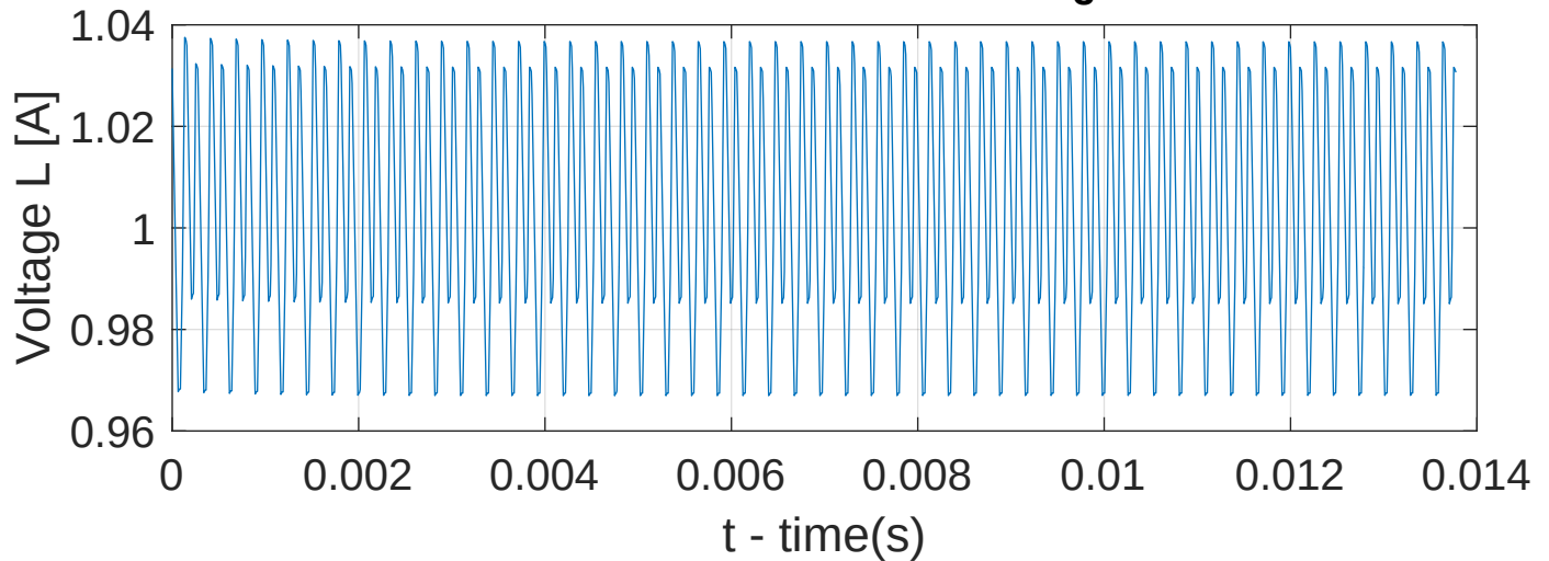
Multilevel Converter: X_3
