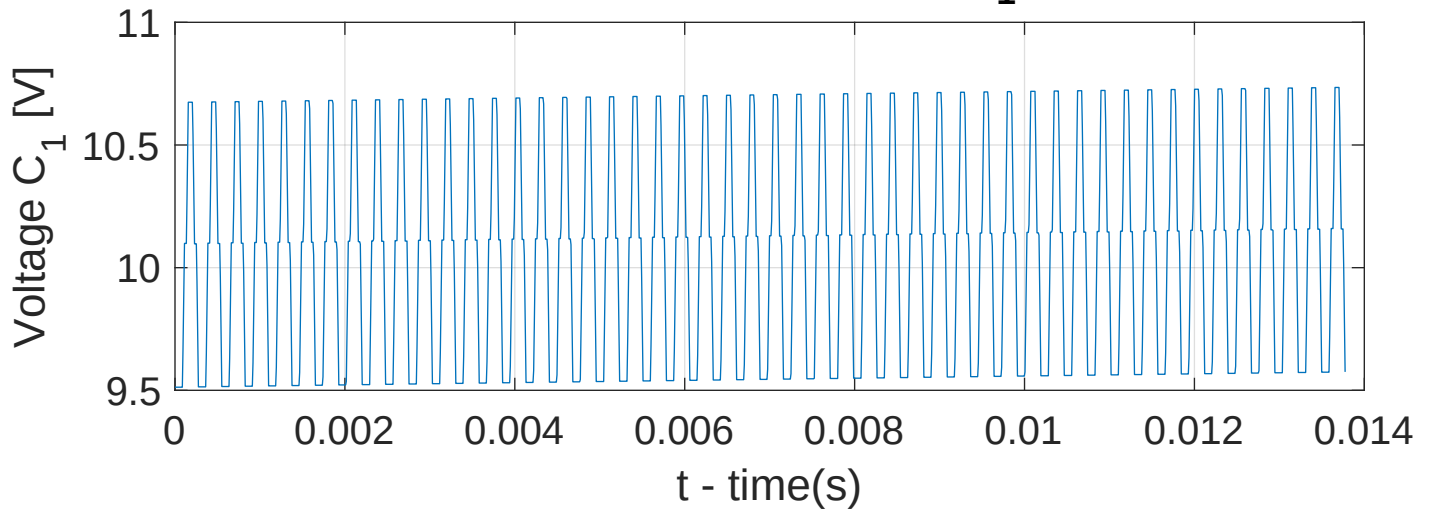
Multilevel Converter: X_2
