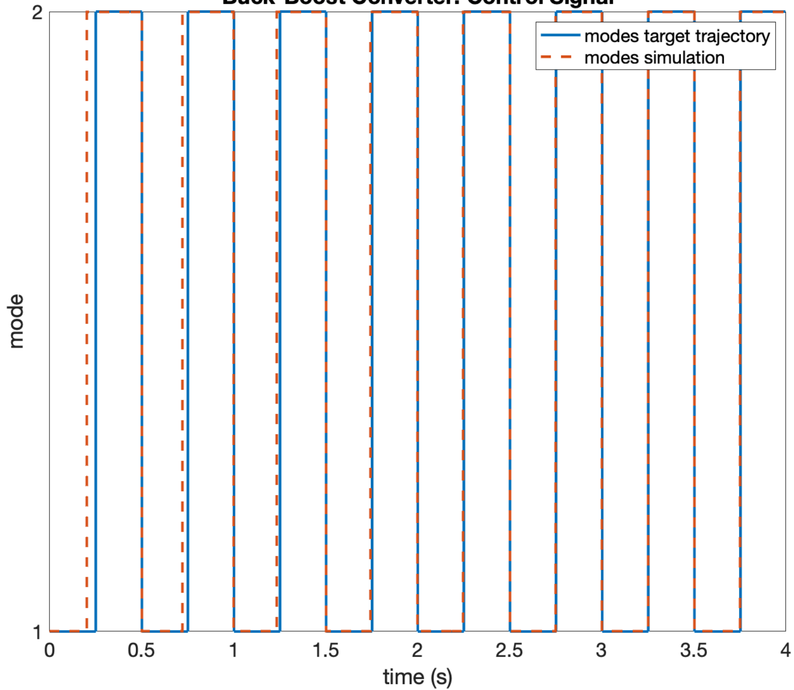
Buck-Boost Converter: Control Signal
