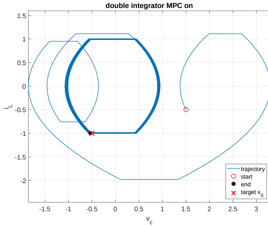
FIGURE 4.4 – State Trajectory MPC on, 50 cycles
