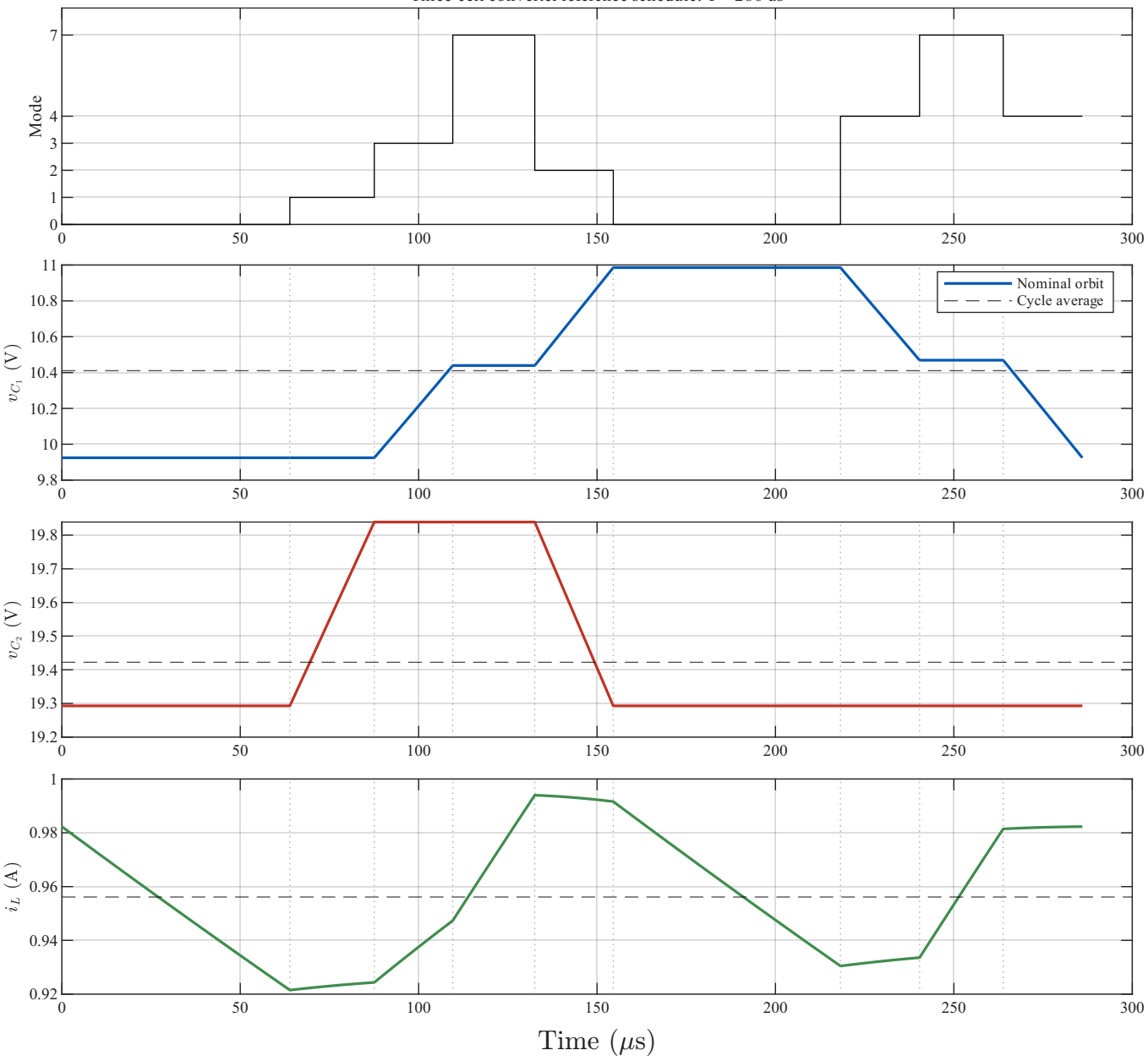
Three-cell converter reference schedule: T = 286 \mu\text{s}
