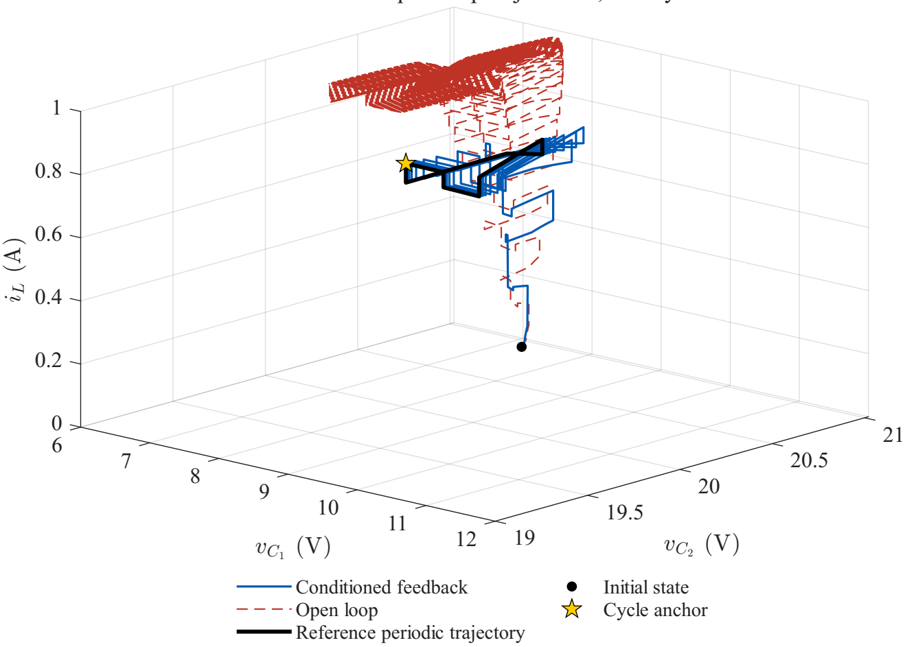
Controlled and open-loop trajectories, 100 cycles
