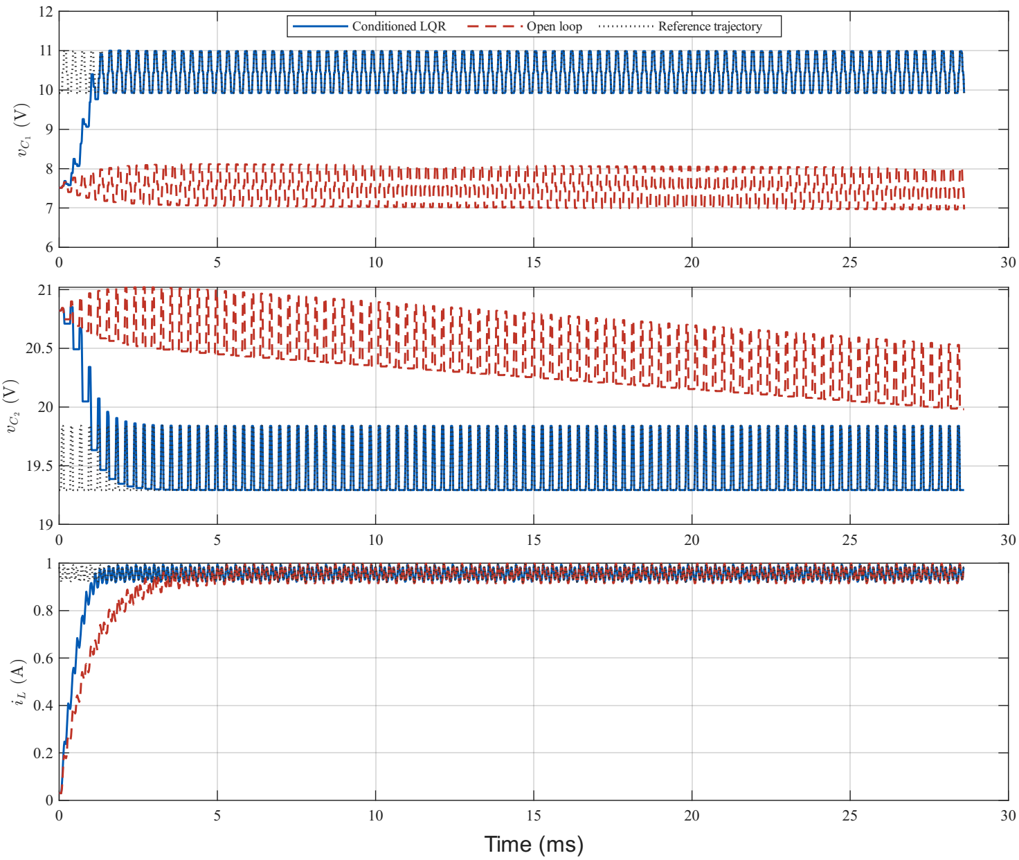
Three-cell converter trajectory comparison over 100 cycles
