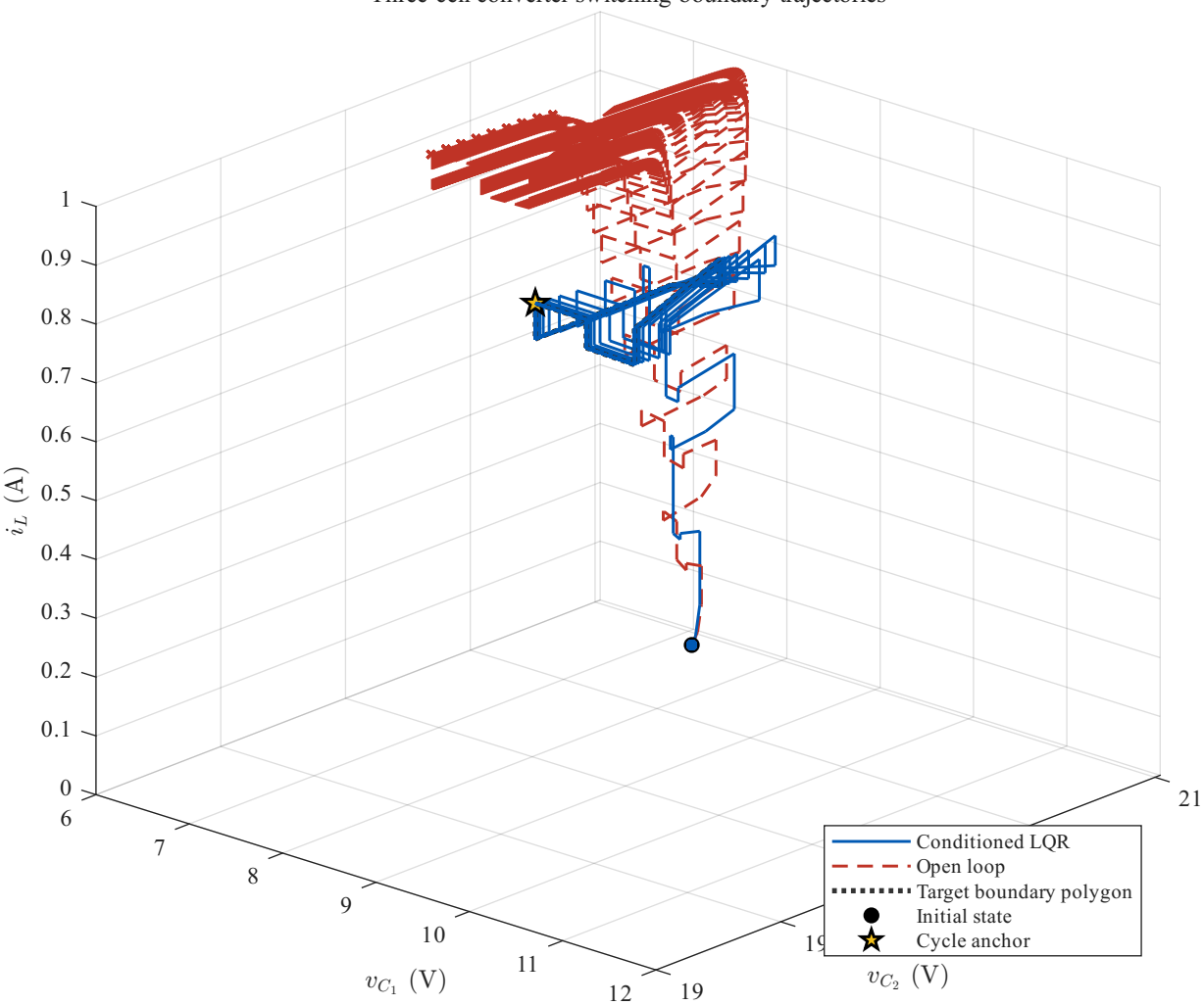
Three-cell converter switching-boundary trajectories
