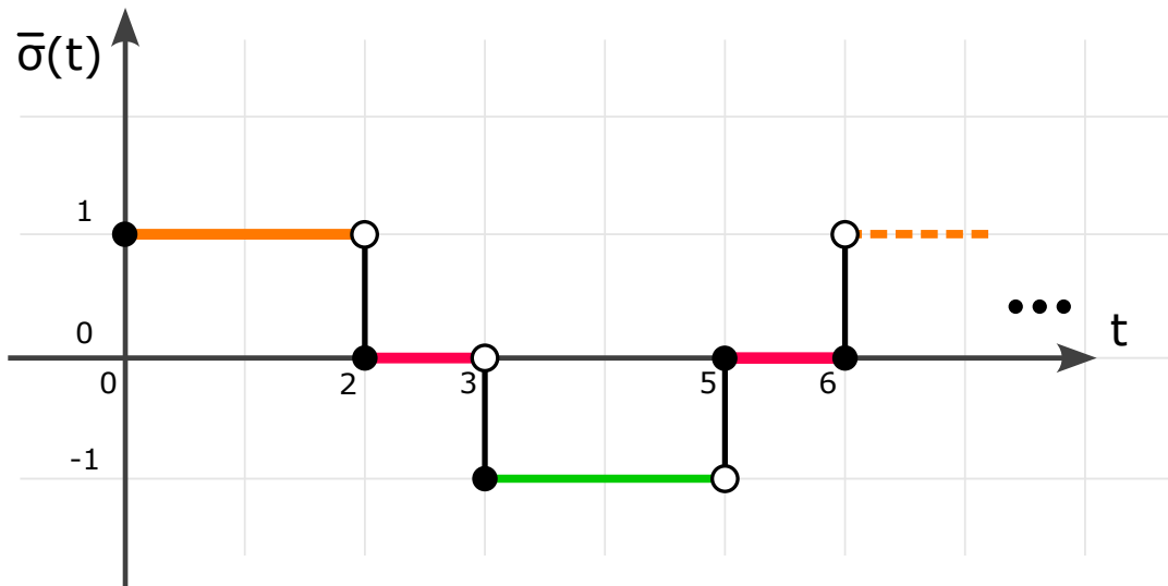
FIGURE 4.2 – Reference signal for Double Integrator
