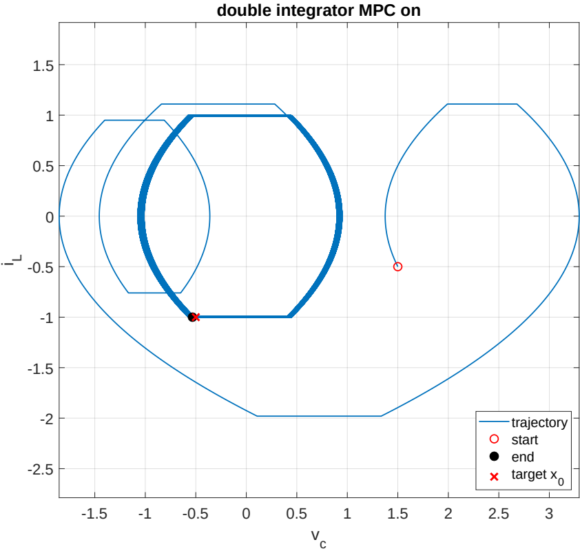
FIGURE 4.4 – State Trajectory MPC on, 50 cycles
