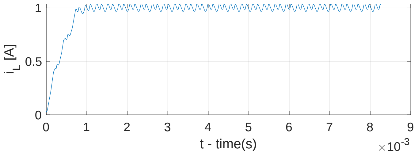
Current i_L Multilevel Converter
