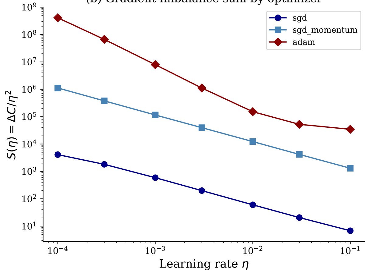
(b) Gradient imbalance sum by optimizer
