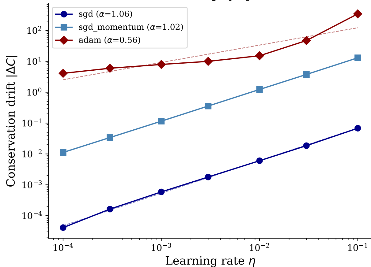
(a) Drift scaling by optimizer
