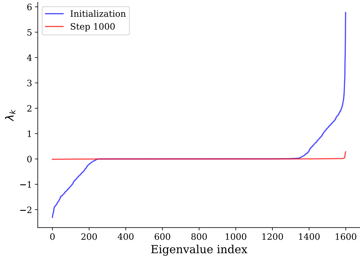
ReLU Hessian spectrum evolution
