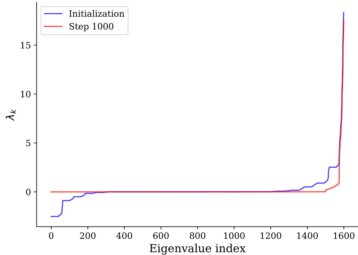
LINEAR Hessian spectrum evolution
