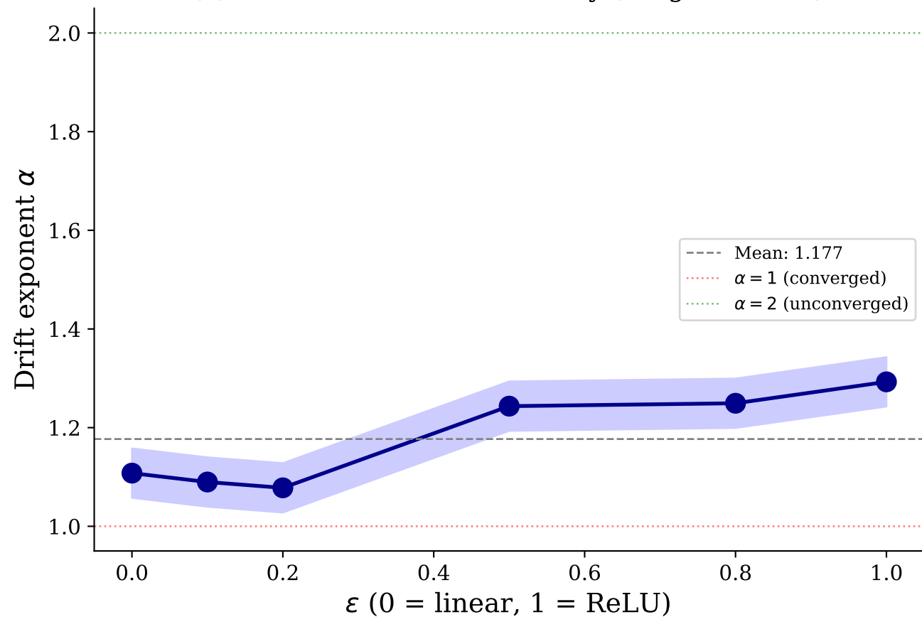
(a) \alpha vs activation nonlinearity (range = 0.215)
