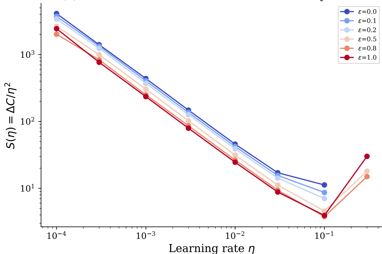
(b) Gradient imbalance sum across nonlinearity levels
