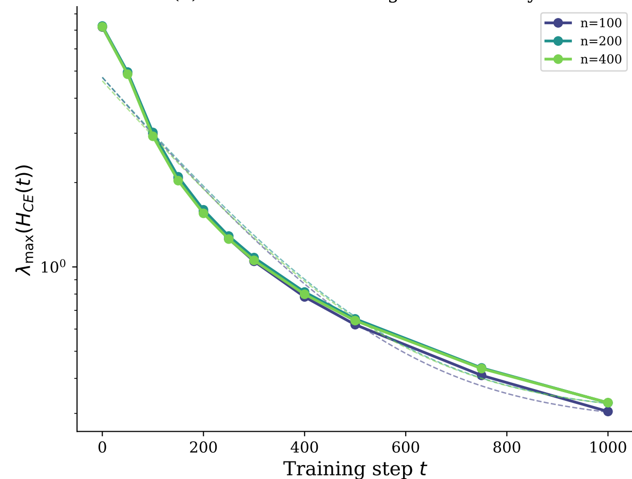
(c) Theorem 5 prediction quality vs Hessian checkpoint
