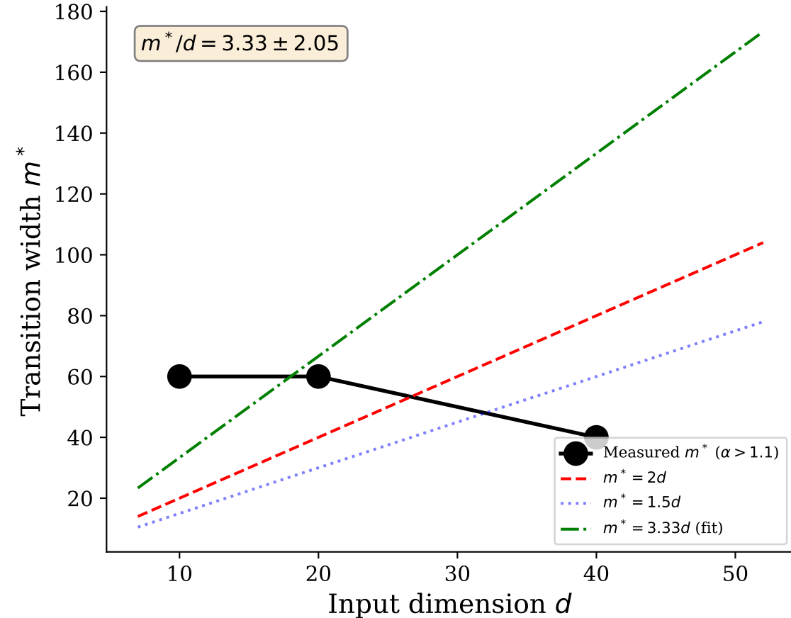
(c) Transition width scales with d
