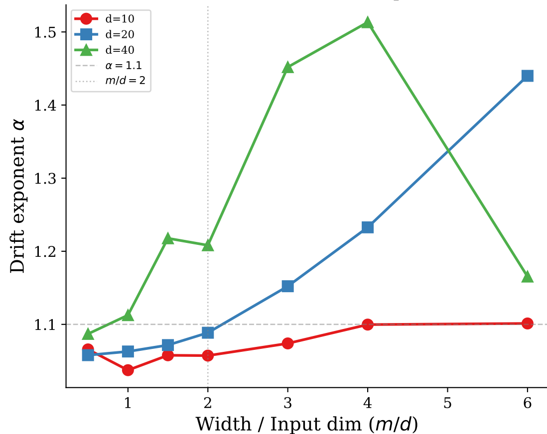
(a) \alpha vs m/d — curve collapse test
