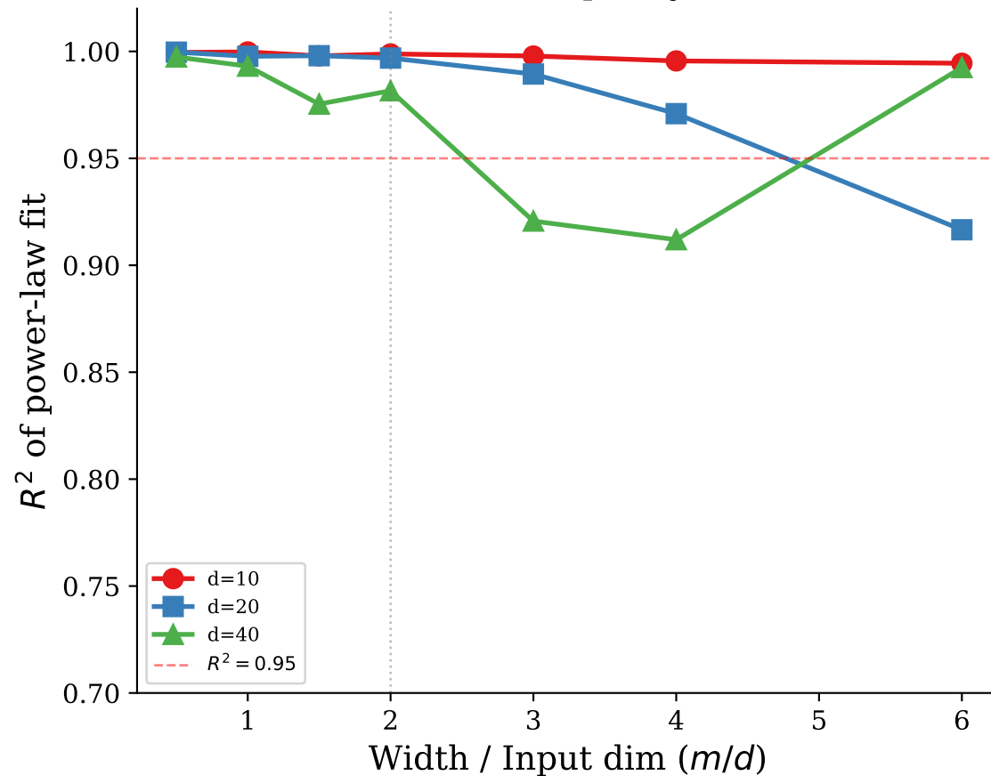
(b) Power-law quality vs m/d
