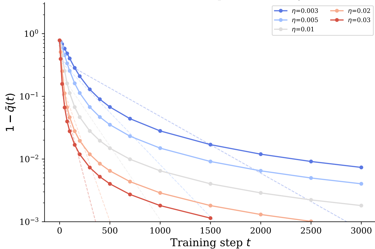
(a) Softmax concentration: exponential decay at rate 1/\tau
