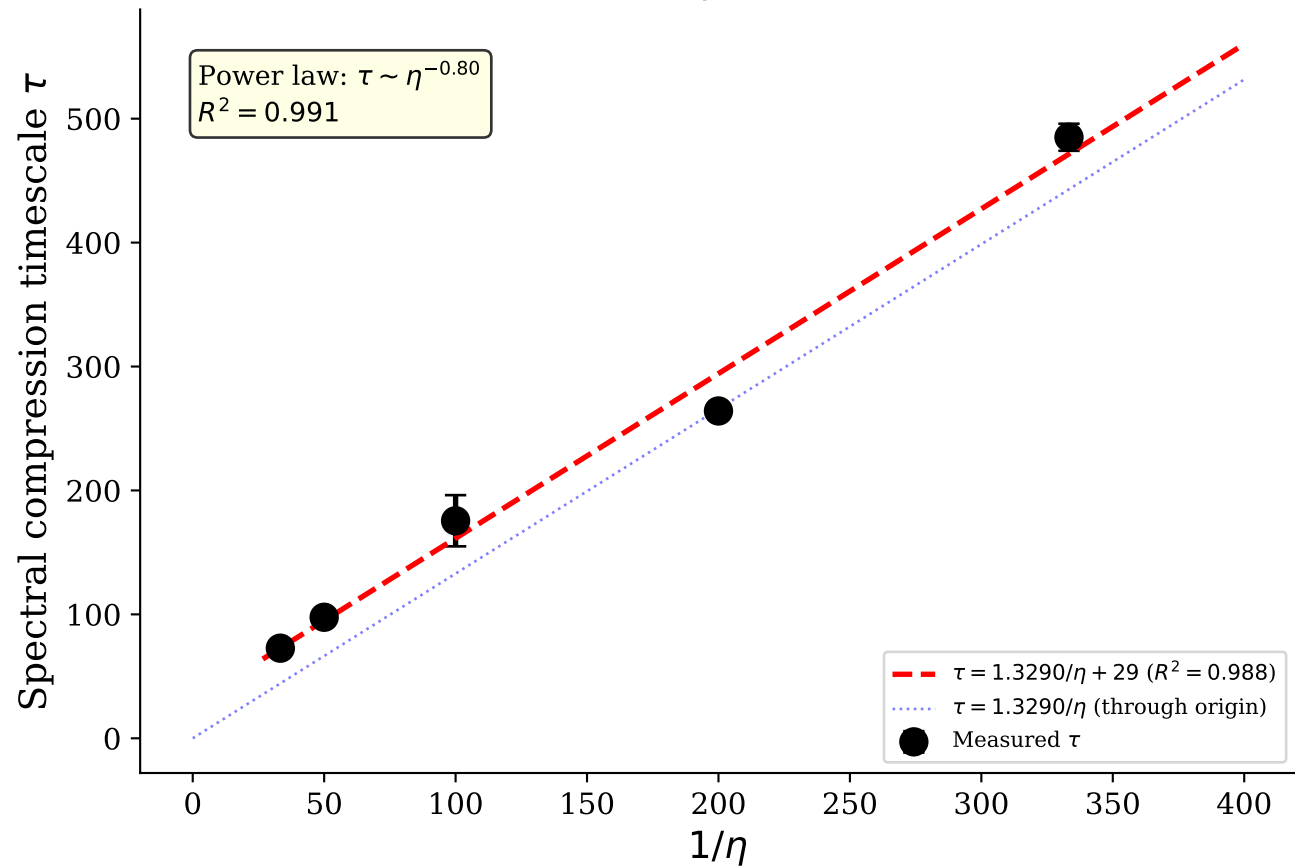
(b) \tau \propto 1/\eta validation
