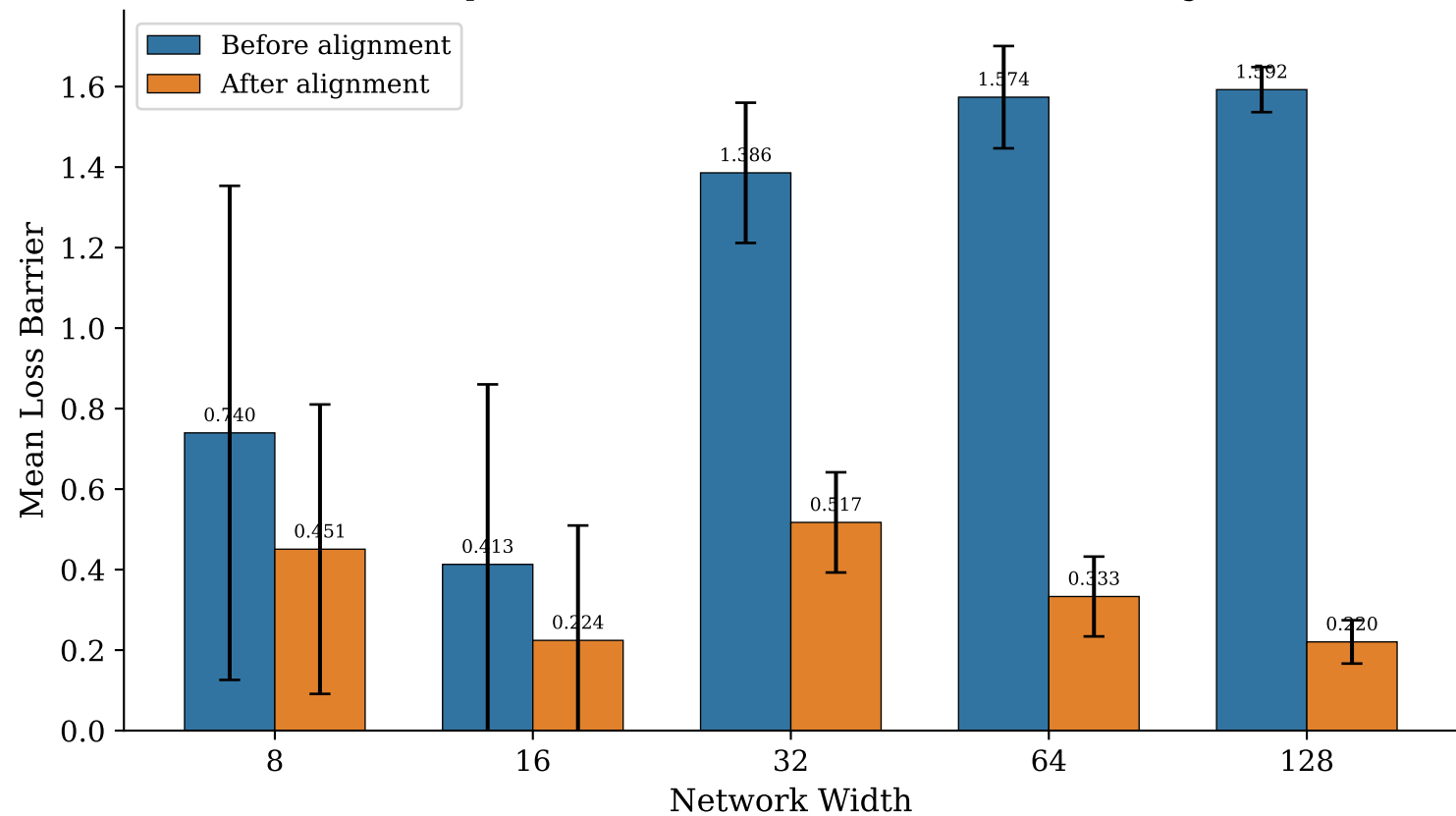
Mode Connectivity: 4-Layer MLP on MNIST (n=1000) Linear Interpolation Barriers Before vs After Permutation Alignment
