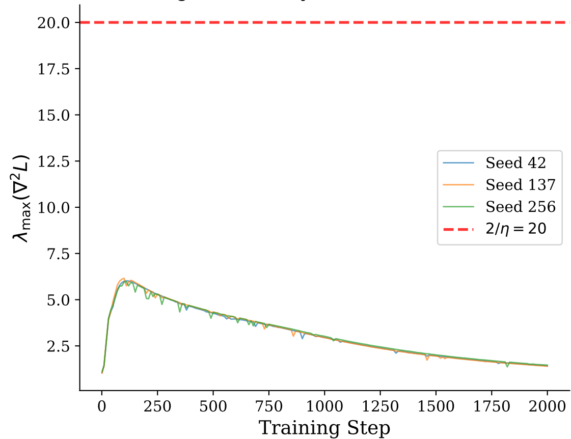
Edge of Stability on MNIST (lr=0.1)
