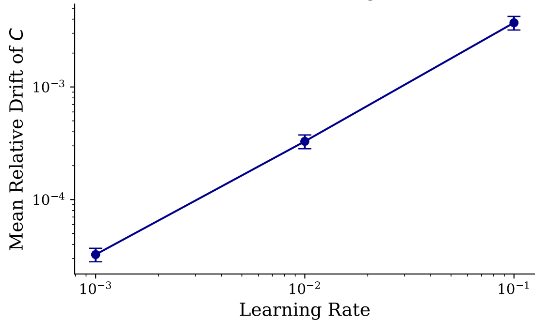
Conservation Drift vs Learning Rate (No Bias)
