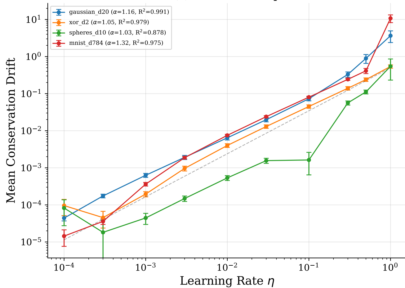
(c) Dataset Sweep
