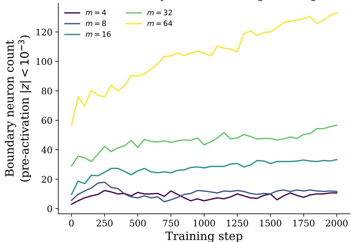
(b) Boundary Neurons During Training
