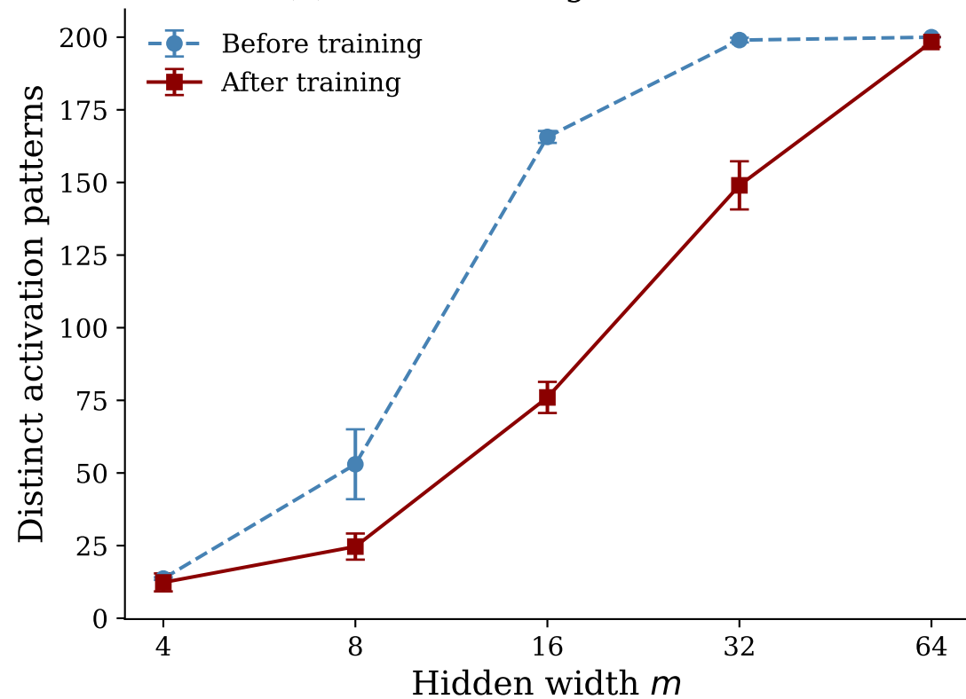
(a) Activation Regions vs Width
