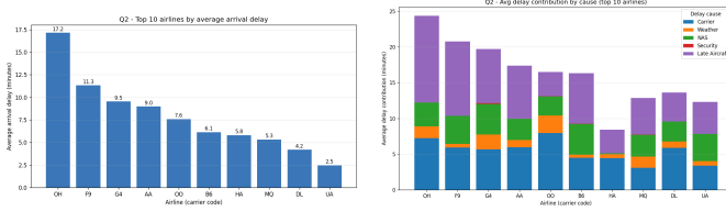
Fig. 3. Q2: top 10 carriers by mean arrival delay (left) and the stacked breakdown of the five delay causes (right). The dominant contributor for the worst-performing carriers is LATE_AIRCRAFT_DELAY, i.e. the cascading effect of aircraft arriving late from a previous leg.
