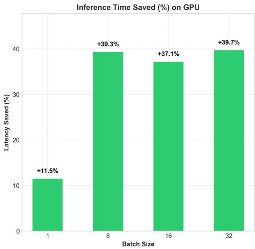
Test set inference Benchmark (GPU & CPU): Model A (24f) (Top-1: 65.85%) vs Cross Frame Model B (16f) (Top-1: 62.68%)
