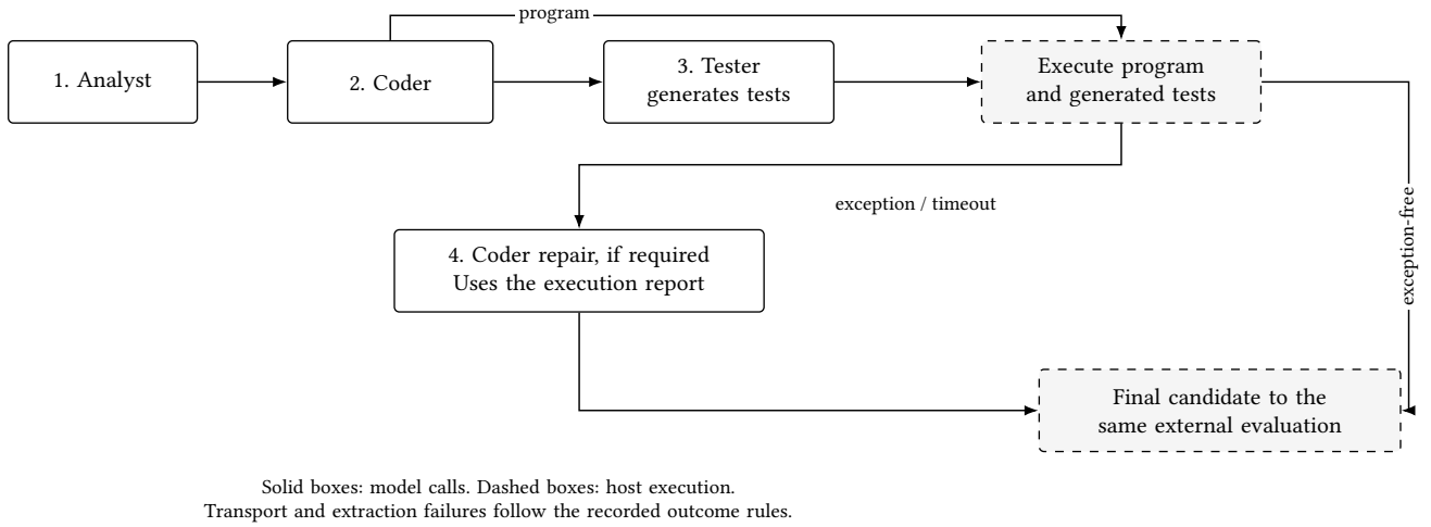
Figure 1: Generation workflows and their evaluation boundary. D, SN, SR, MN and MR are the five factorial conditions. In a separate contemporaneous study, SCC is compared with fresh SN and SR using the same model. SCC’s generated tests are not the hidden benchmark tests. The diagram shows ordinary completion paths; transport aborts and author-code extraction fallbacks are handled separately. An exception-free internal run does not establish benchmark correctness. The configured SCC controller does not retest a repaired program internally.
