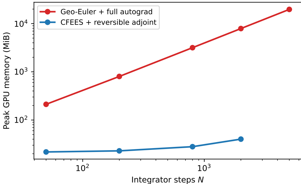
SDE integrator memory vs. N \sim S^{15} , batch=64 (RTX 4060 Laptop)
