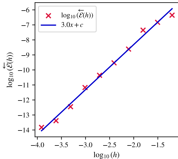
\overleftarrow{\mathcal{E}}(h) for EES(2,7)
